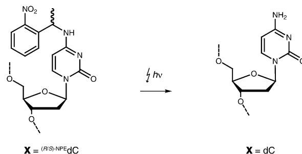
Scheme 1. The investigated DNA sequence contains a photolabile modification at the central cytosine nucleobase. The structure of the NPE-modified nucleotide is depicted below. Upon light irradiation, the unmodified sequence is recovered.
